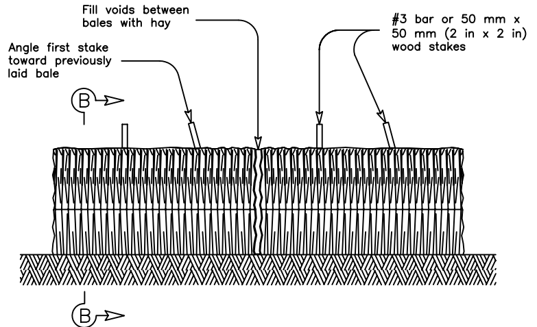
BALED HAY FOR EROSION CONTROL
