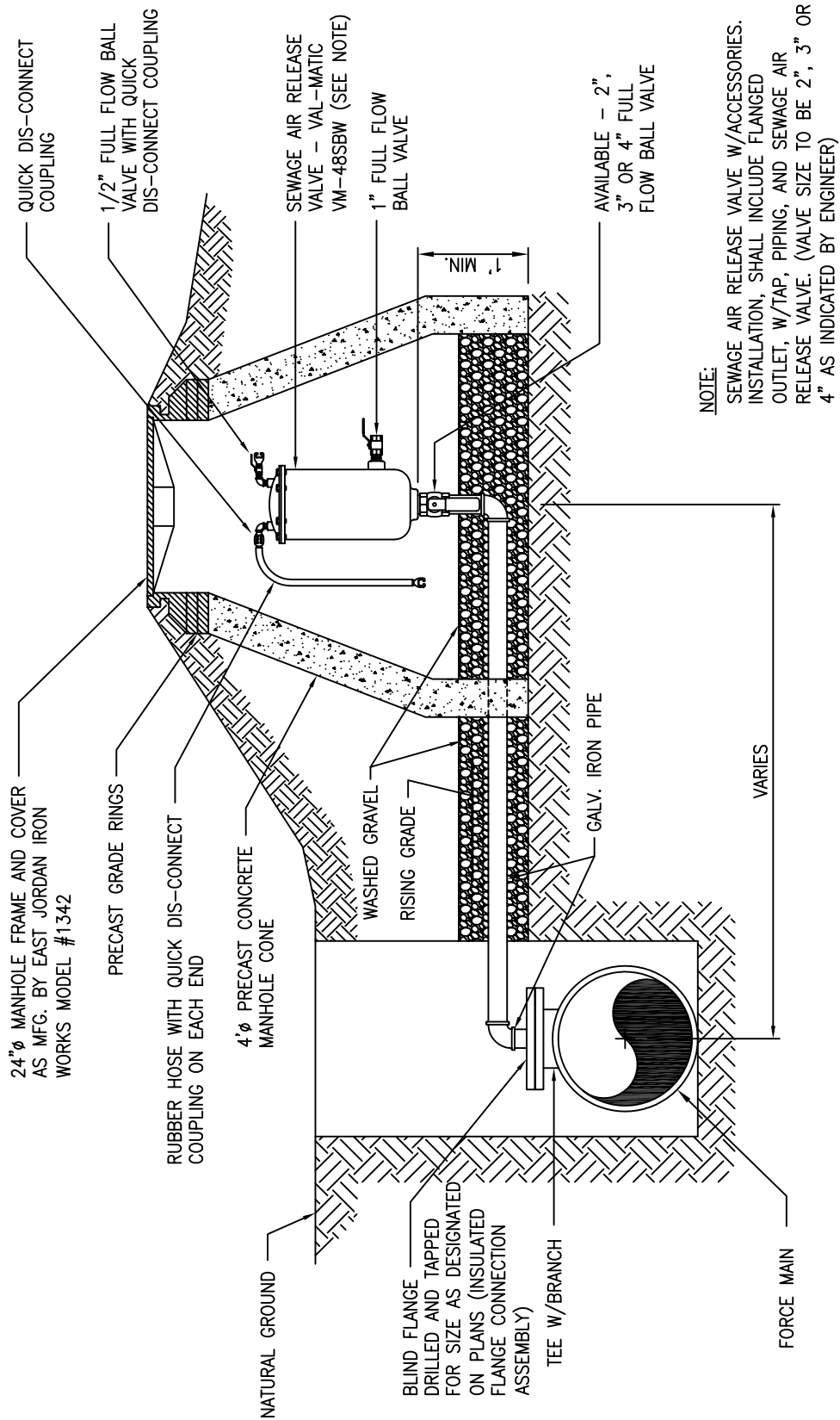
10_SSCS_AIR_RELEASE_VALVE.Dwg
