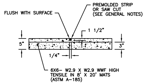
TYPE B CONTRACTION JOINT
