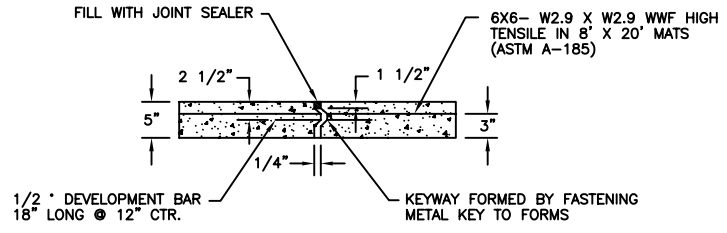
TYPE C LONGITUDINAL CONSTRUCTION JOINT
